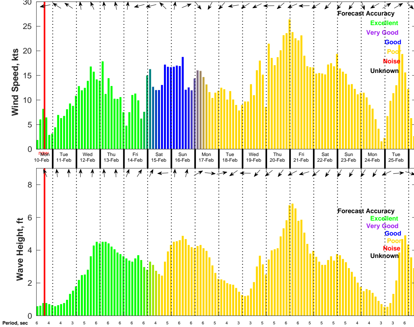
Wind & Wave Forecast for NDBC 42036 from 10-Feb-2025 07:00:00 to 26-Feb-2025 07:00:00
