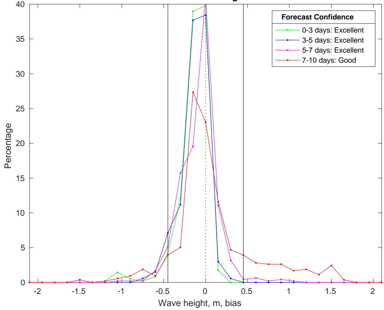
NDBC 42040 vs CMEMS Waves Bias Histogram: 10-Feb-2025
