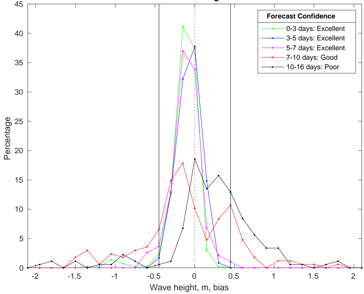
NDBC 42040 vs GFS Waves Bias Histogram: 10-Feb-2025
