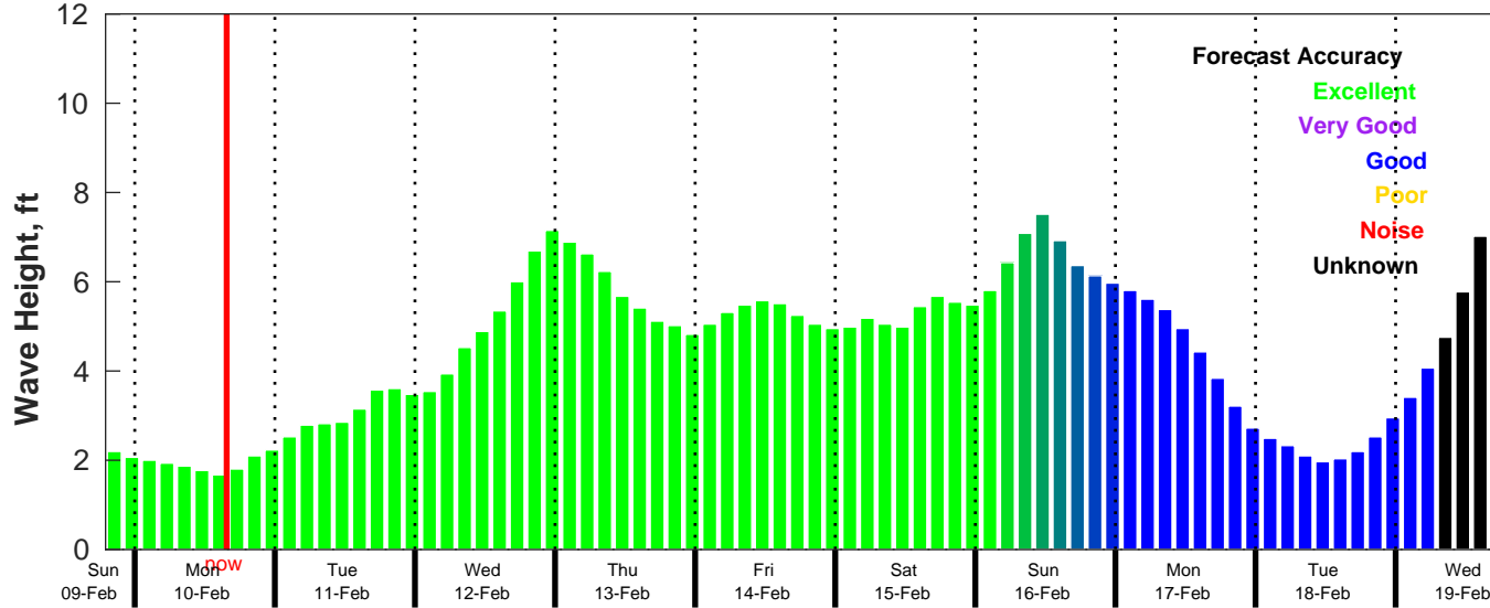
CMEMS Wave Forecast for NDBC 42040 from 09-Feb-2025 19:00:00 to 19-Feb-2025 19:00:00
