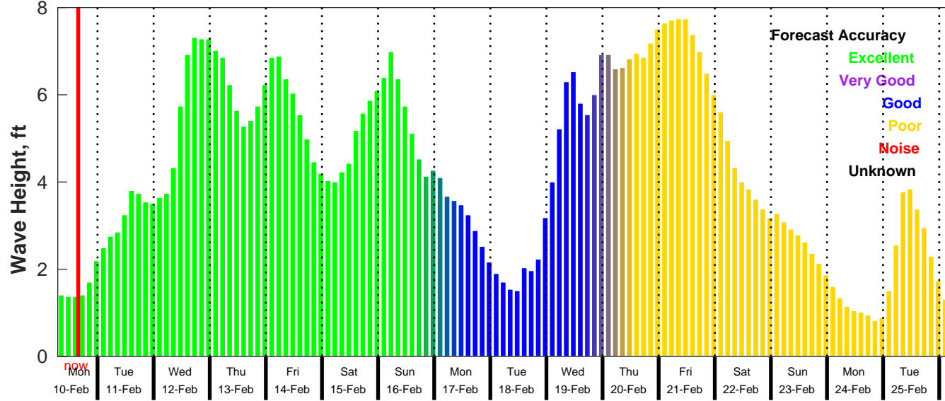
GFS Wave Forecast for NDBC 42040 from 10-Feb-2025 07:00:00 to 26-Feb-2025 07:00:00
