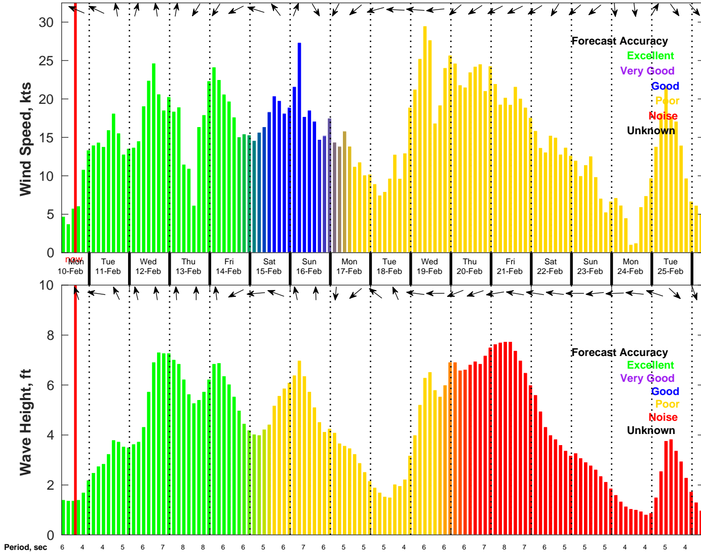
Wind & Wave Forecast for NDBC 42040 from 10-Feb-2025 07:00:00 to 26-Feb-2025 07:00:00
