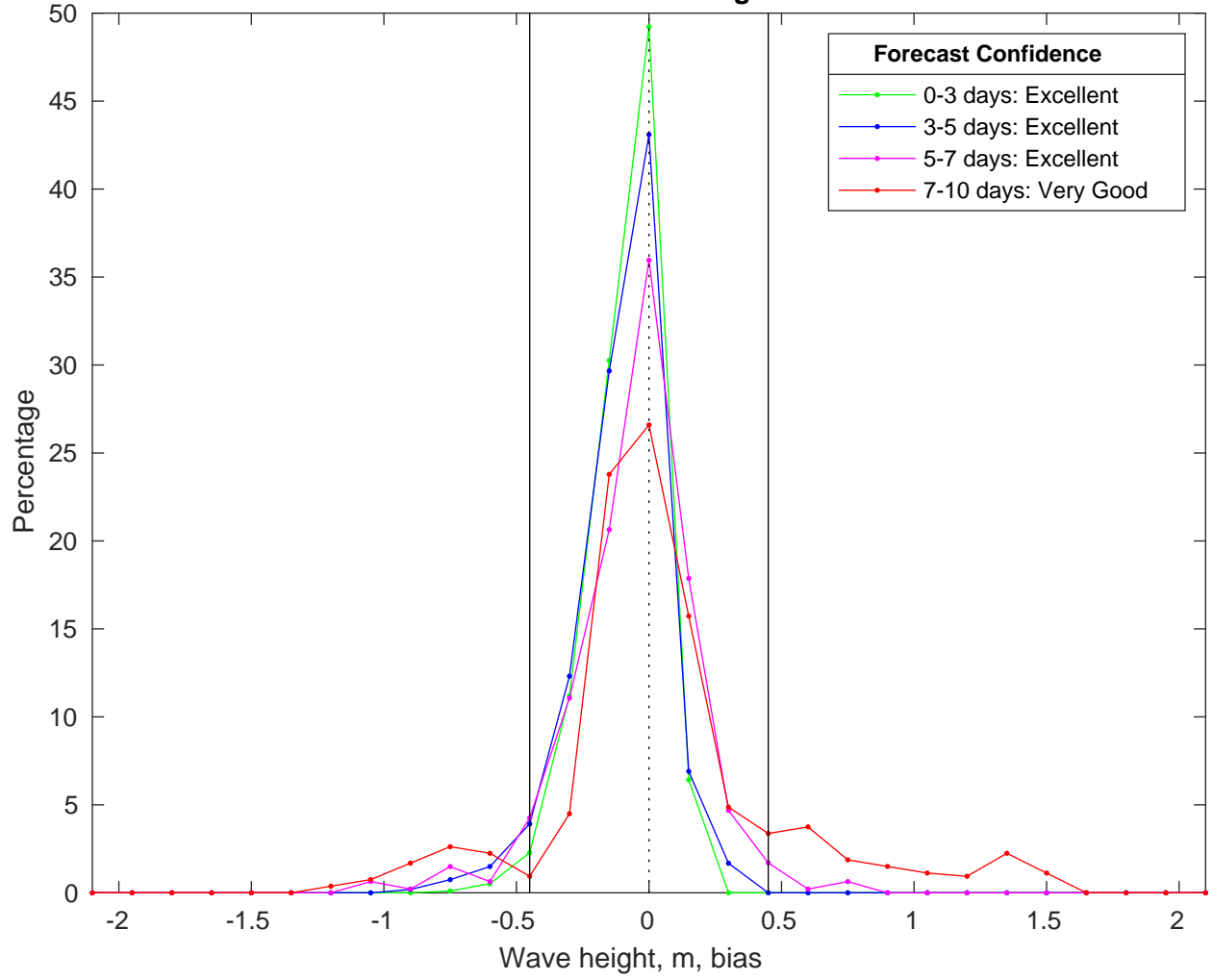
NDBC 42084 vs CMEMS Waves Bias Histogram: 10-Feb-2025
