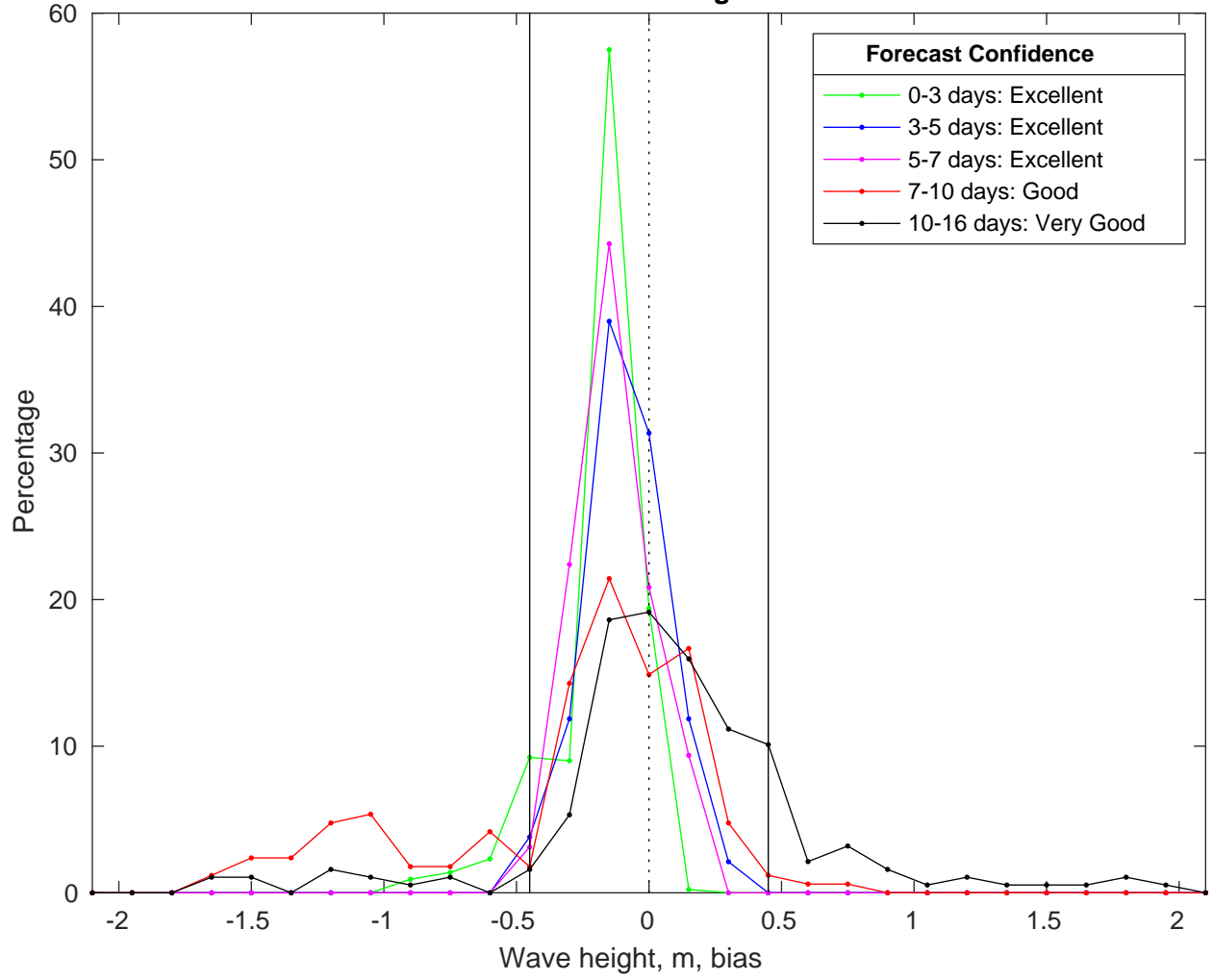
NDBC 42084 vs GFS Waves Bias Histogram: 10-Feb-2025
