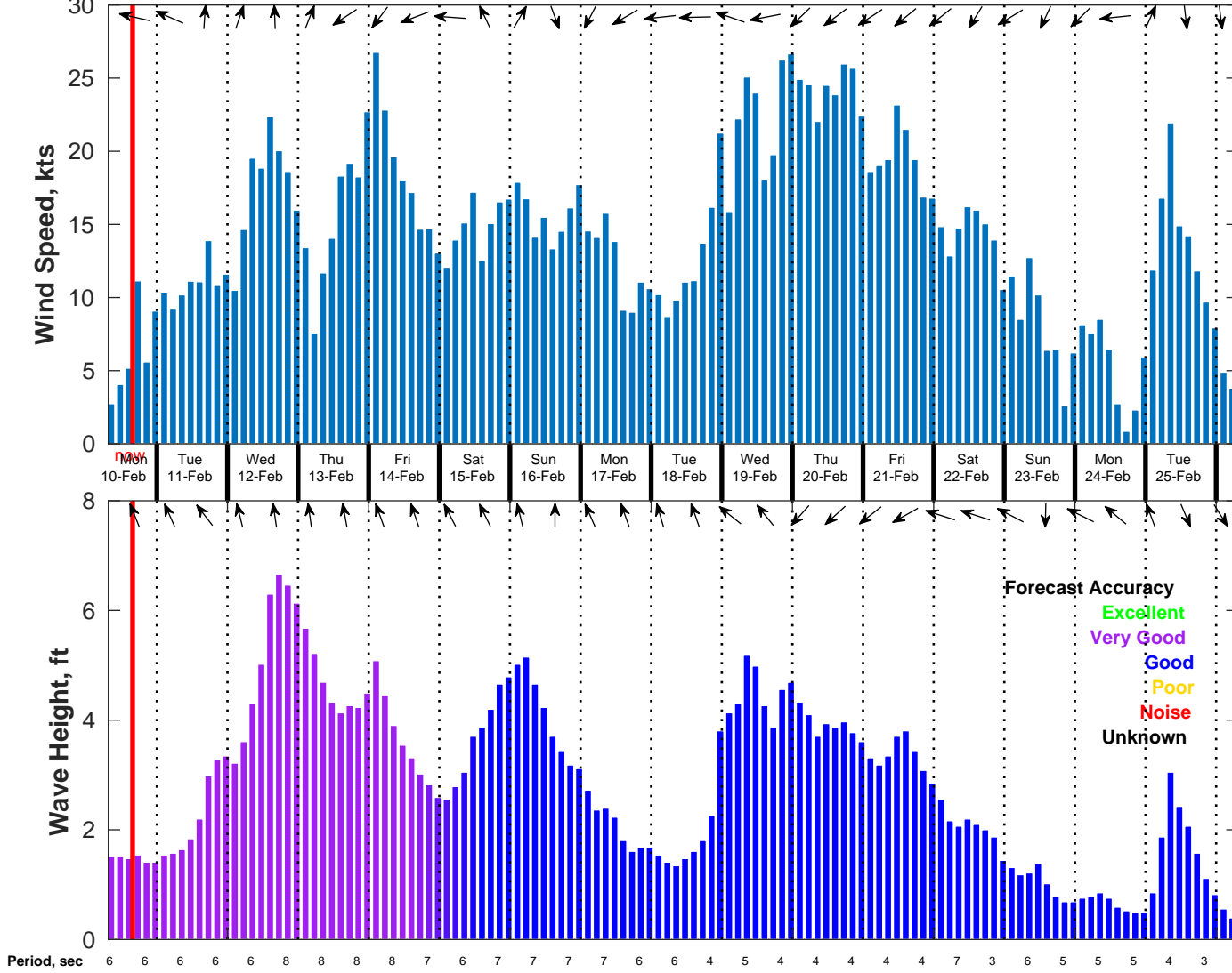
Wind & Wave Forecast for NDBC 42084 from 10-Feb-2025 07:00:00 to 26-Feb-2025 07:00:00
