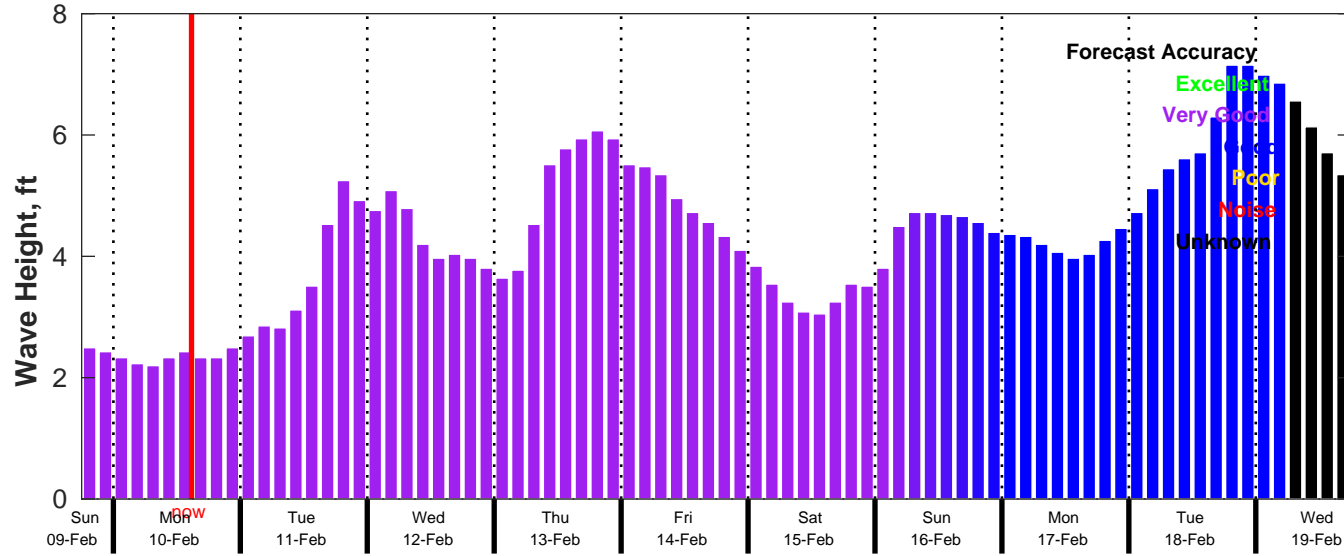
CMEMS Wave Forecast for NDBC 42092 from 09-Feb-2025 18:00:00 to 19-Feb-2025 18:00:00
