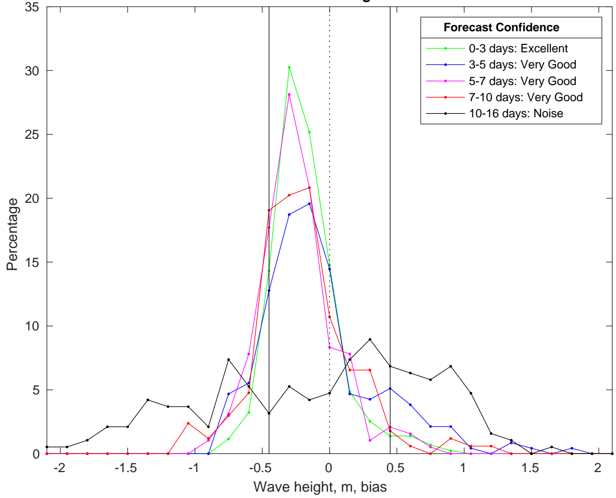
NDBC 46011 vs GFS Waves Bias Histogram: 10-Feb-2025
