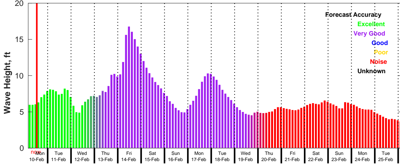
GFS Wave Forecast for NDBC 46011 from 10-Feb-2025 04:00:00 to 26-Feb-2025 04:00:00
