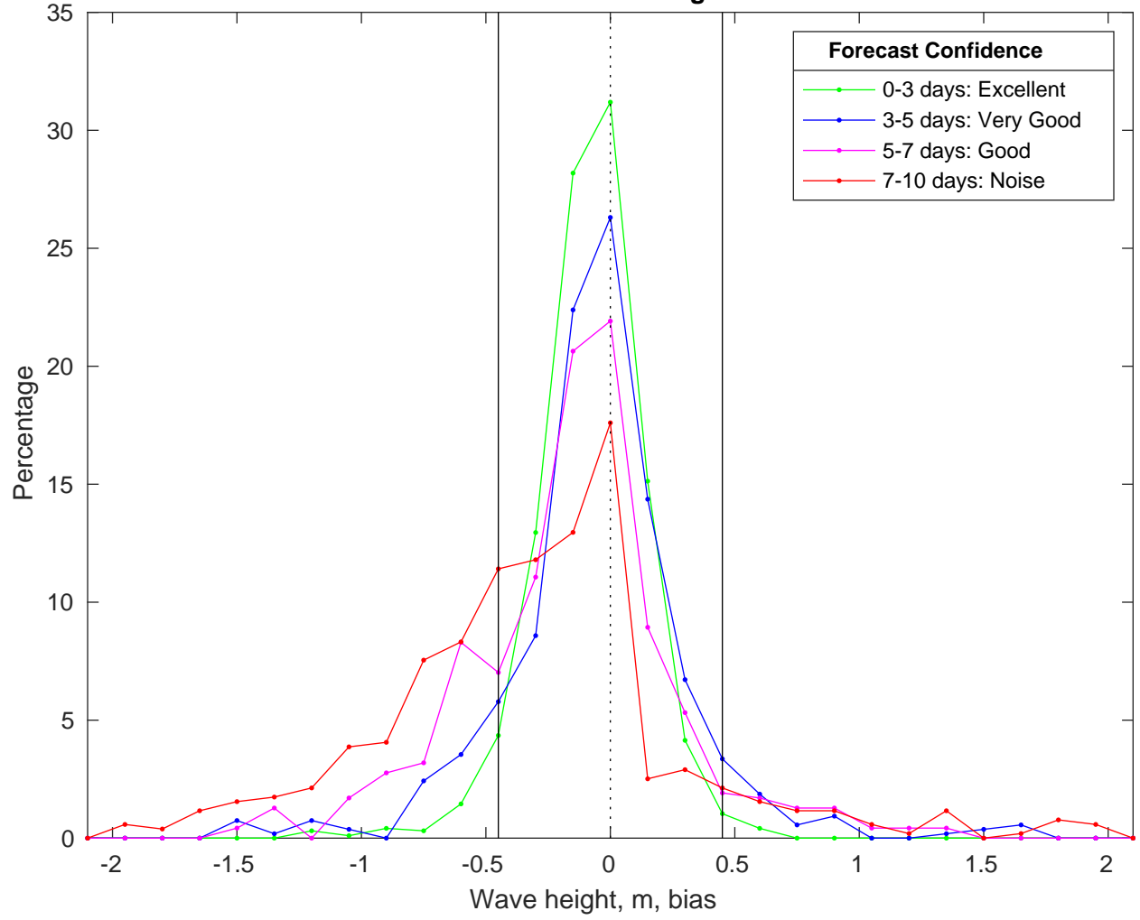
NDBC 46028 vs CMEMS Waves Bias Histogram: 10-Feb-2025
