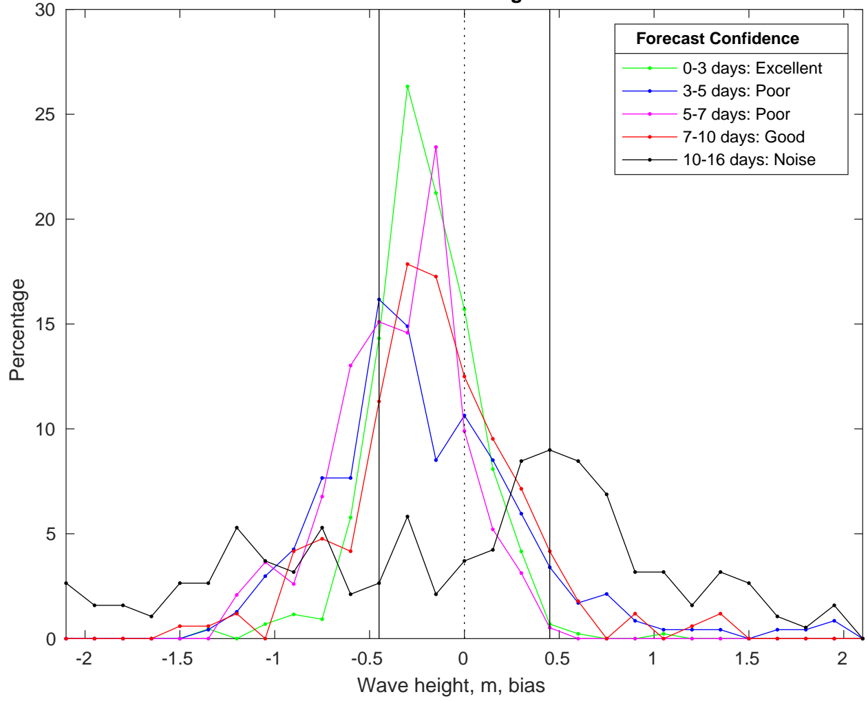
NDBC 46028 vs GFS Waves Bias Histogram: 10-Feb-2025
