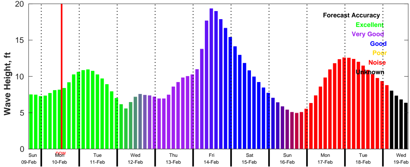
CMEMS Wave Forecast for NDBC 46028 from 09-Feb-2025 16:00:00 to 19-Feb-2025 16:00:00
