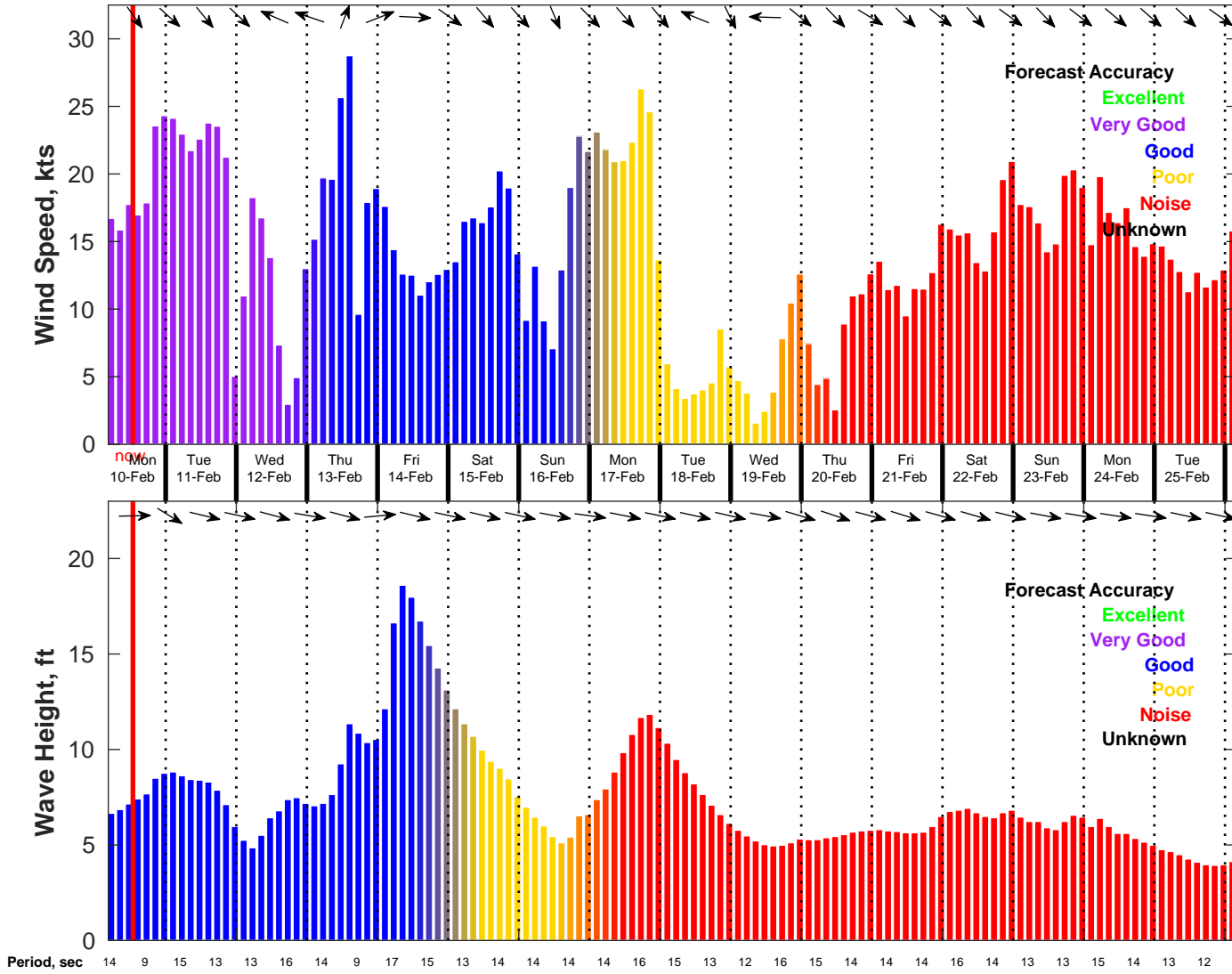
Wind & Wave Forecast for NDBC 46028 from 10-Feb-2025 04:00:00 to 26-Feb-2025 04:00:00
