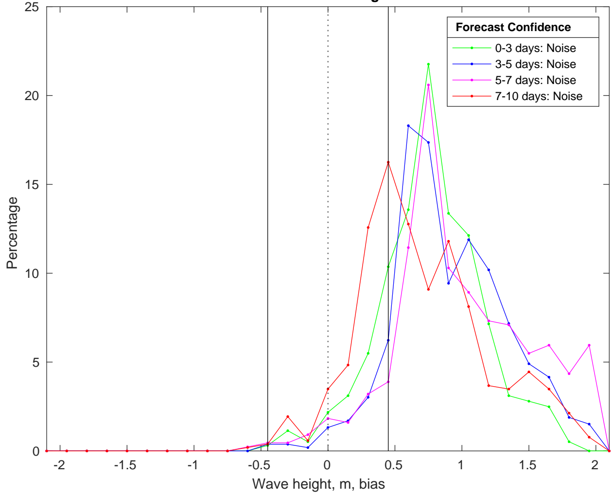
NDBC 46053 vs CMEMS Waves Bias Histogram: 10-Feb-2025
