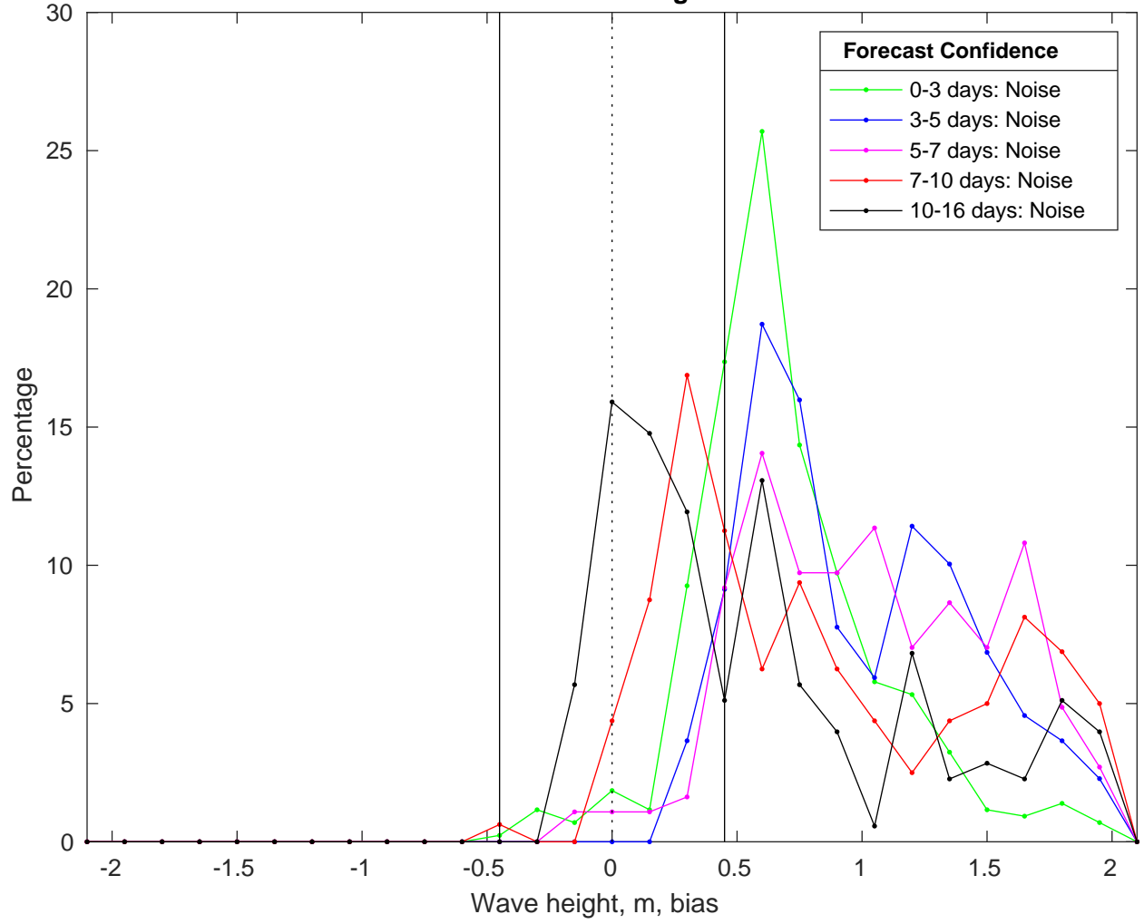
NDBC 46053 vs GFS Waves Bias Histogram: 10-Feb-2025
