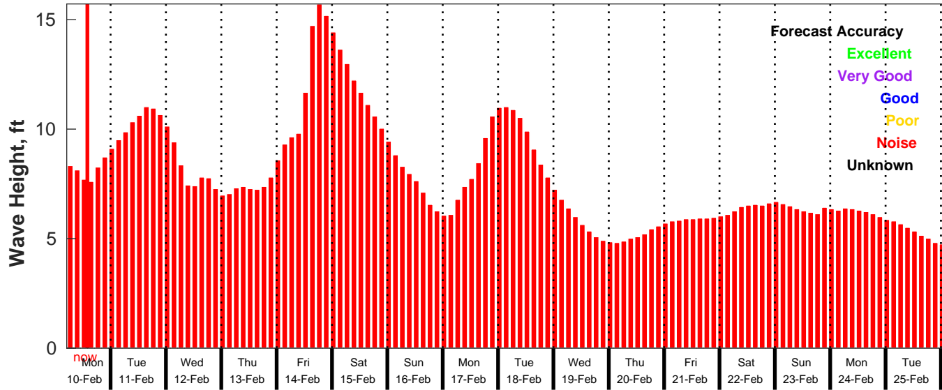
GFS Wave Forecast for NDBC 46053 from 10-Feb-2025 05:00:00 to 26-Feb-2025 05:00:00
