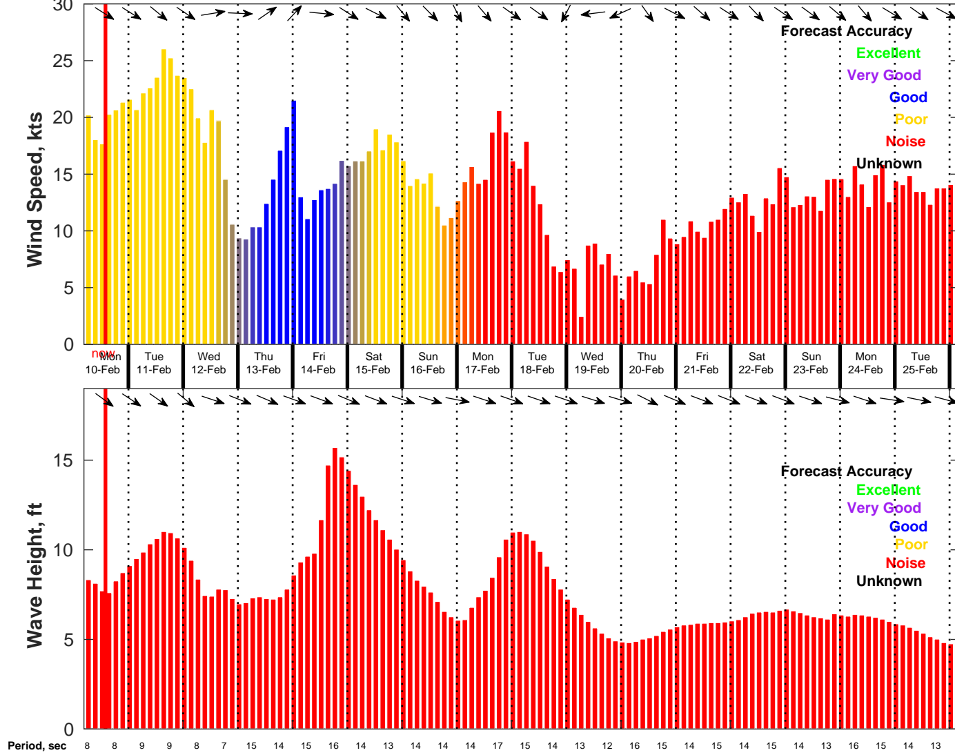
Wind & Wave Forecast for NDBC 46053 from 10-Feb-2025 05:00:00 to 26-Feb-2025 05:00:00
