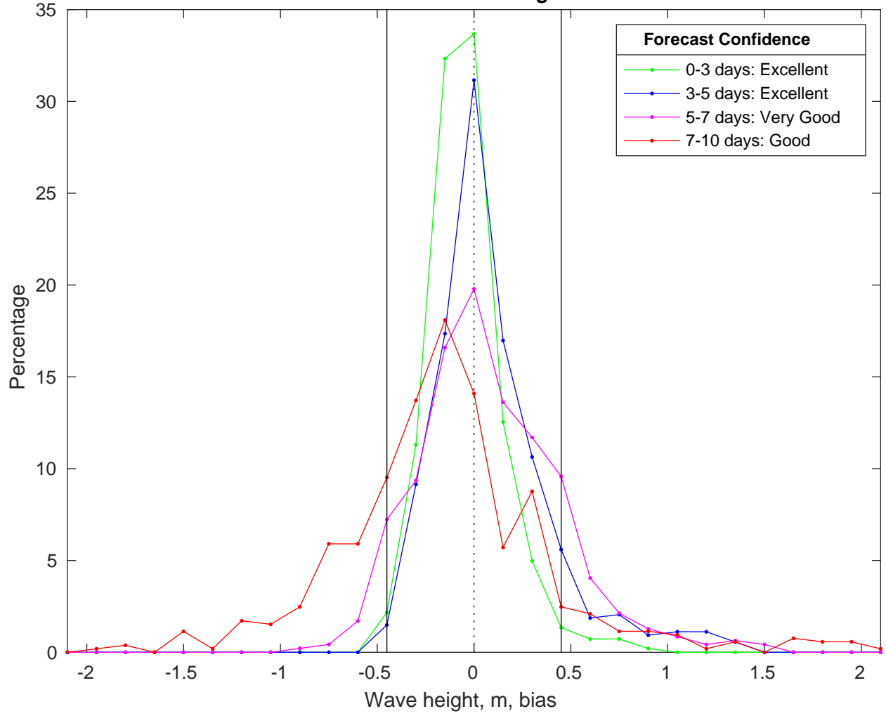
NDBC 46054 vs CMEMS Waves Bias Histogram: 10-Feb-2025
