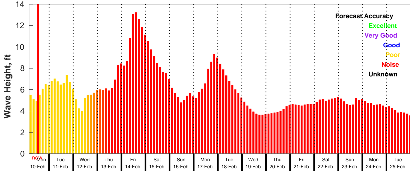
GFS Wave Forecast for NDBC 46054 from 10-Feb-2025 04:00:00 to 26-Feb-2025 04:00:00
