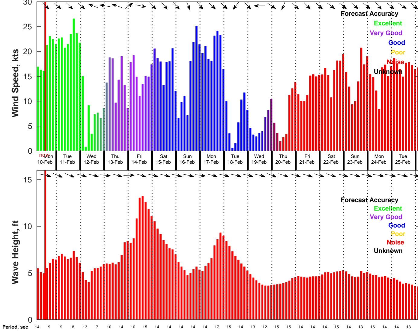
Wind & Wave Forecast for NDBC 46054 from 10-Feb-2025 04:00:00 to 26-Feb-2025 04:00:00
