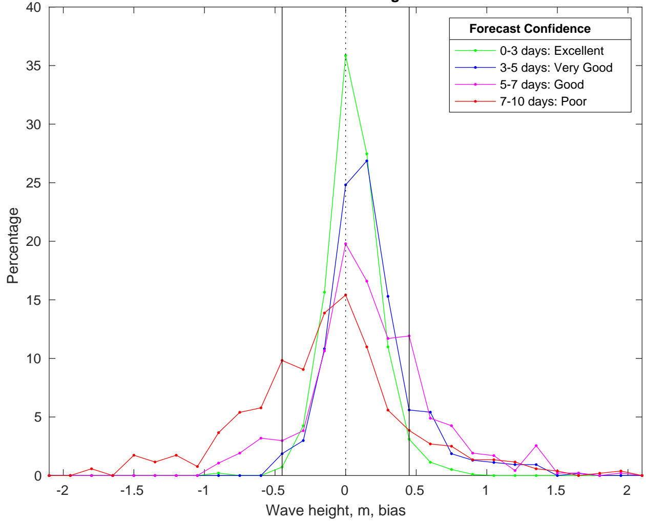
NDBC 46069 vs CMEMS Waves Bias Histogram: 10-Feb-2025
