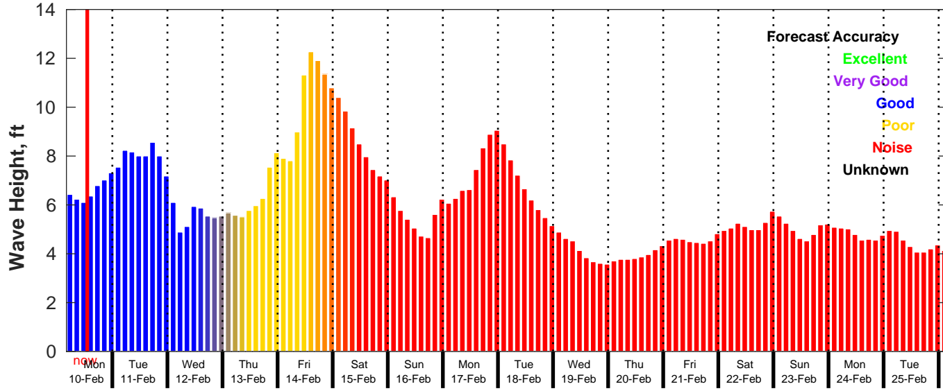
GFS Wave Forecast for NDBC 46069 from 10-Feb-2025 04:00:00 to 26-Feb-2025 04:00:00
