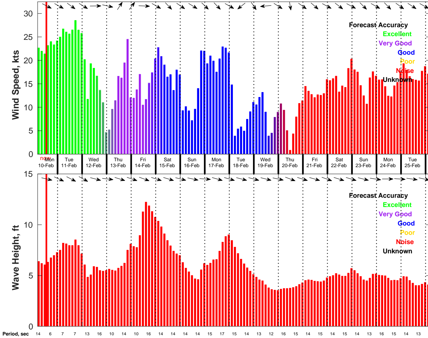
Wind & Wave Forecast for NDBC 46069 from 10-Feb-2025 04:00:00 to 26-Feb-2025 04:00:00
