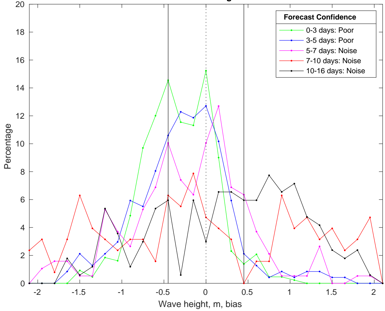
NDBC 46246 vs GFS Waves Bias Histogram: 10-Feb-2025
