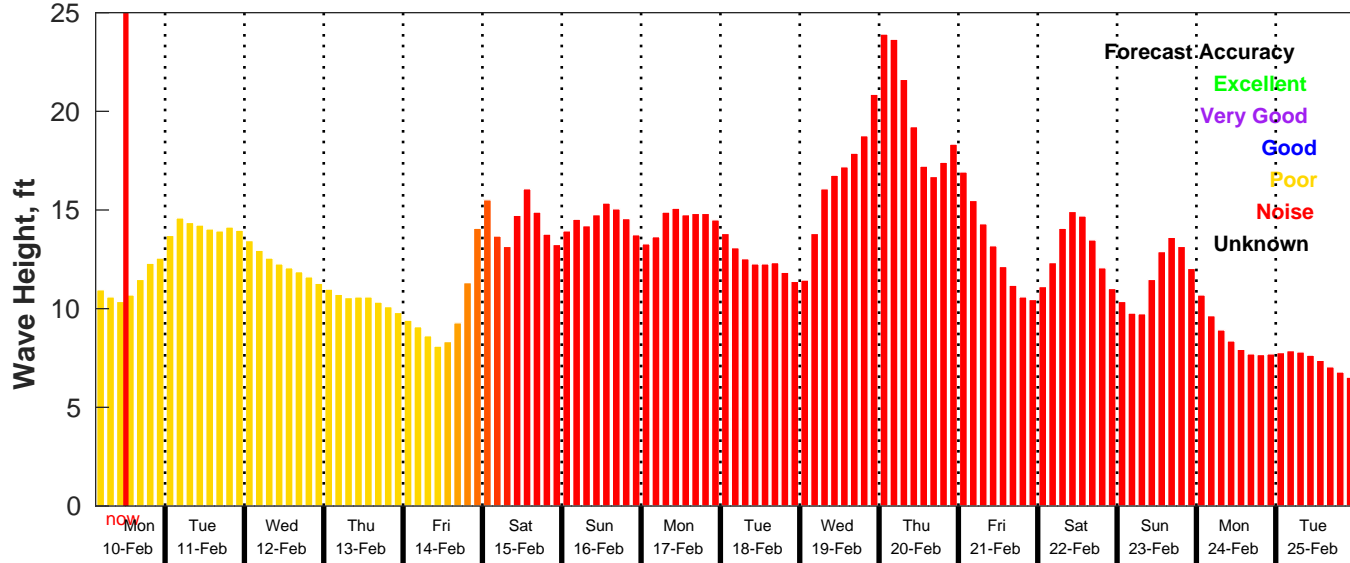
GFS Wave Forecast for NDBC 46246 from 10-Feb-2025 03:00:00 to 26-Feb-2025 03:00:00
