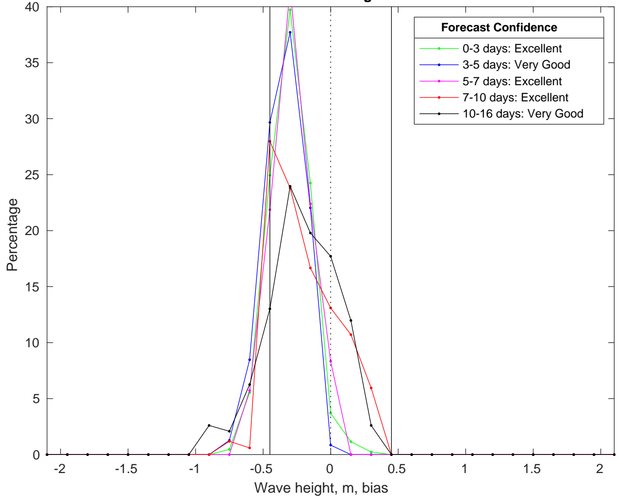
NDBC 51209 vs GFS Waves Bias Histogram: 10-Feb-2025
