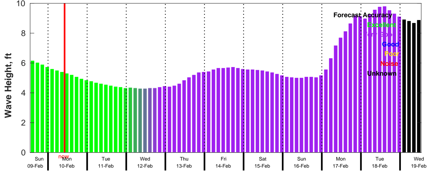
CMEMS Wave Forecast for NDBC 51209 from 09-Feb-2025 13:00:00 to 19-Feb-2025 13:00:00
