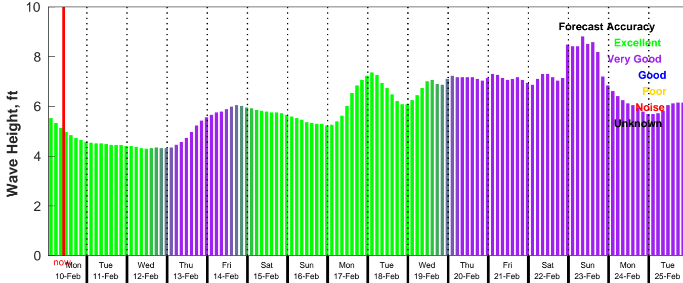
GFS Wave Forecast for NDBC 51209 from 10-Feb-2025 01:00:00 to 26-Feb-2025 01:00:00
