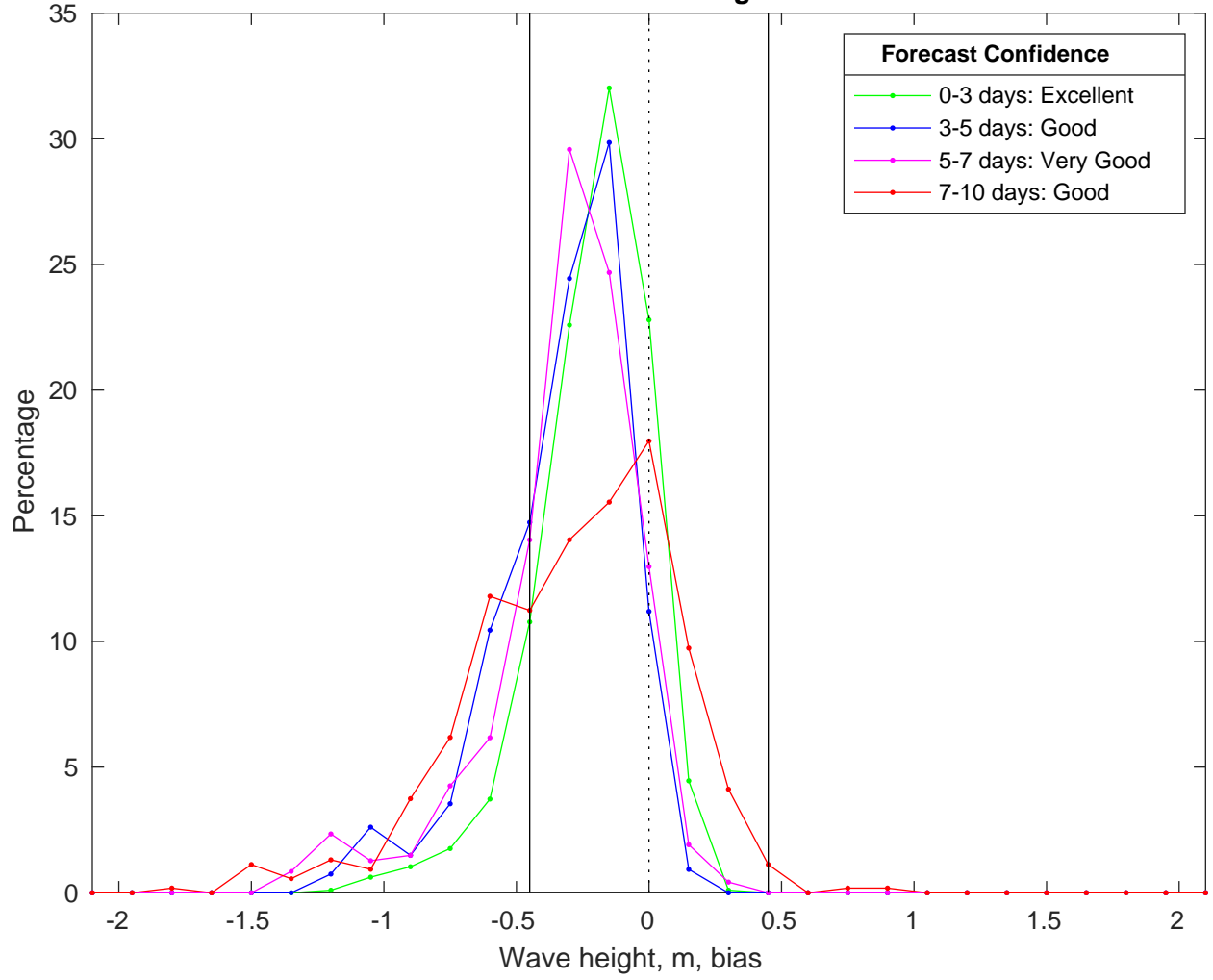
NDBC 52211 vs CMEMS Waves Bias Histogram: 10-Feb-2025
