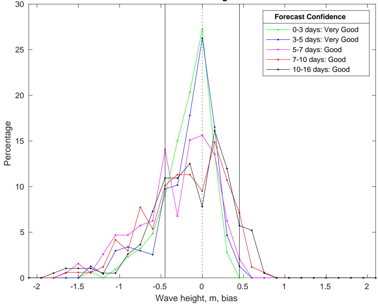
NDBC 52211 vs GFS Waves Bias Histogram: 10-Feb-2025
