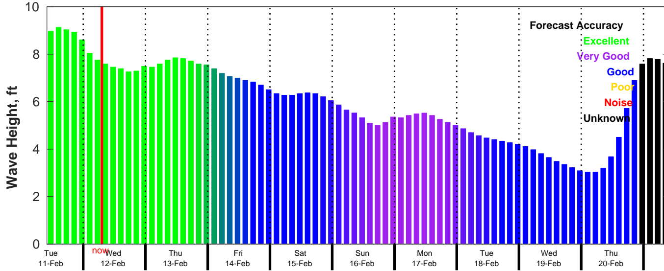
CMEMS Wave Forecast for NDBC 52211 from 10-Feb-2025 10:00:00 to 20-Feb-2025 10:00:00
