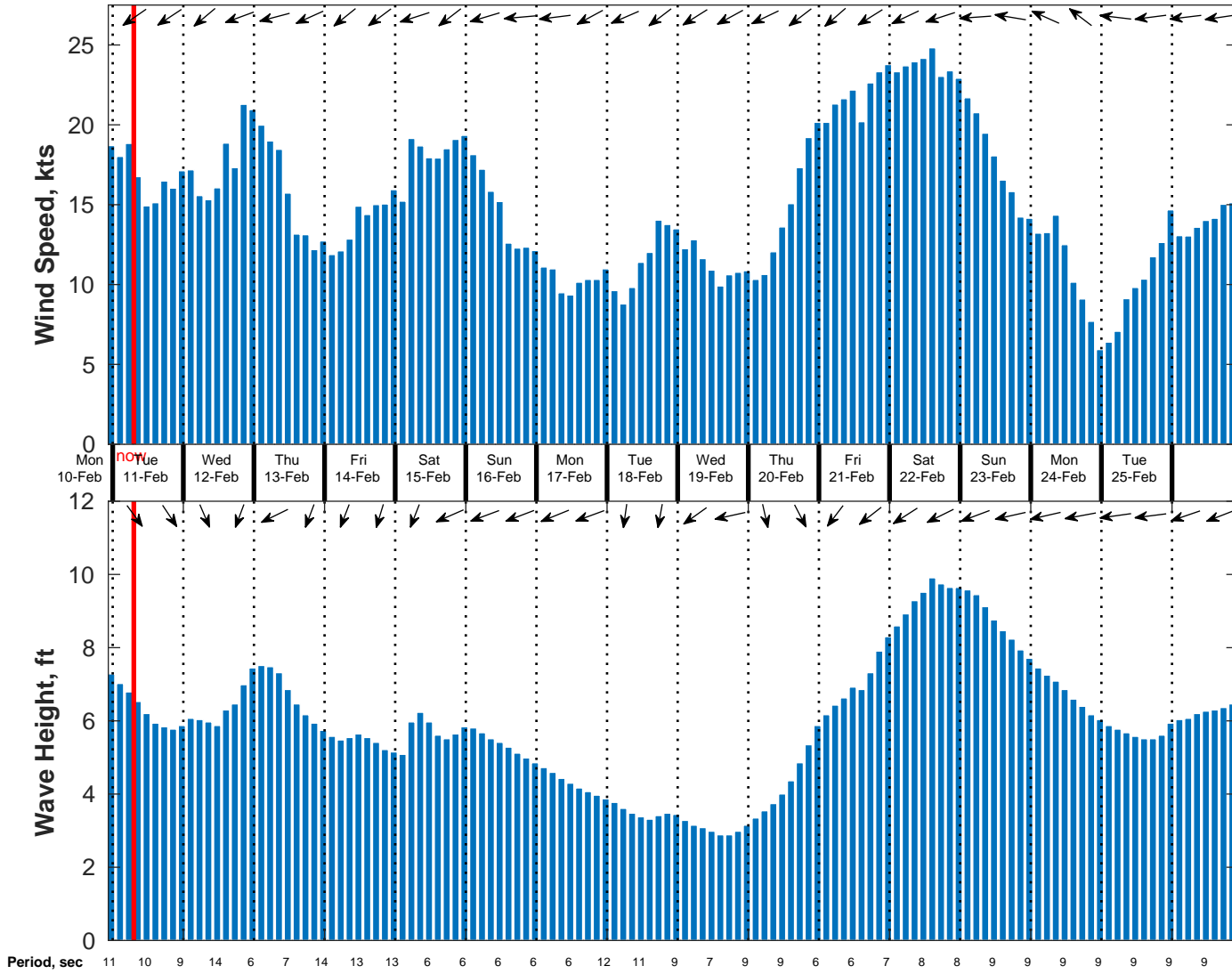
Wind & Wave Forecast for NDBC 52211 from 10-Feb-2025 22:00:00 to 26-Feb-2025 22:00:00
