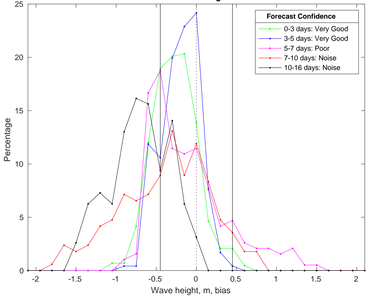
NDBC 52212 vs GFS Waves Bias Histogram: 10-Feb-2025
