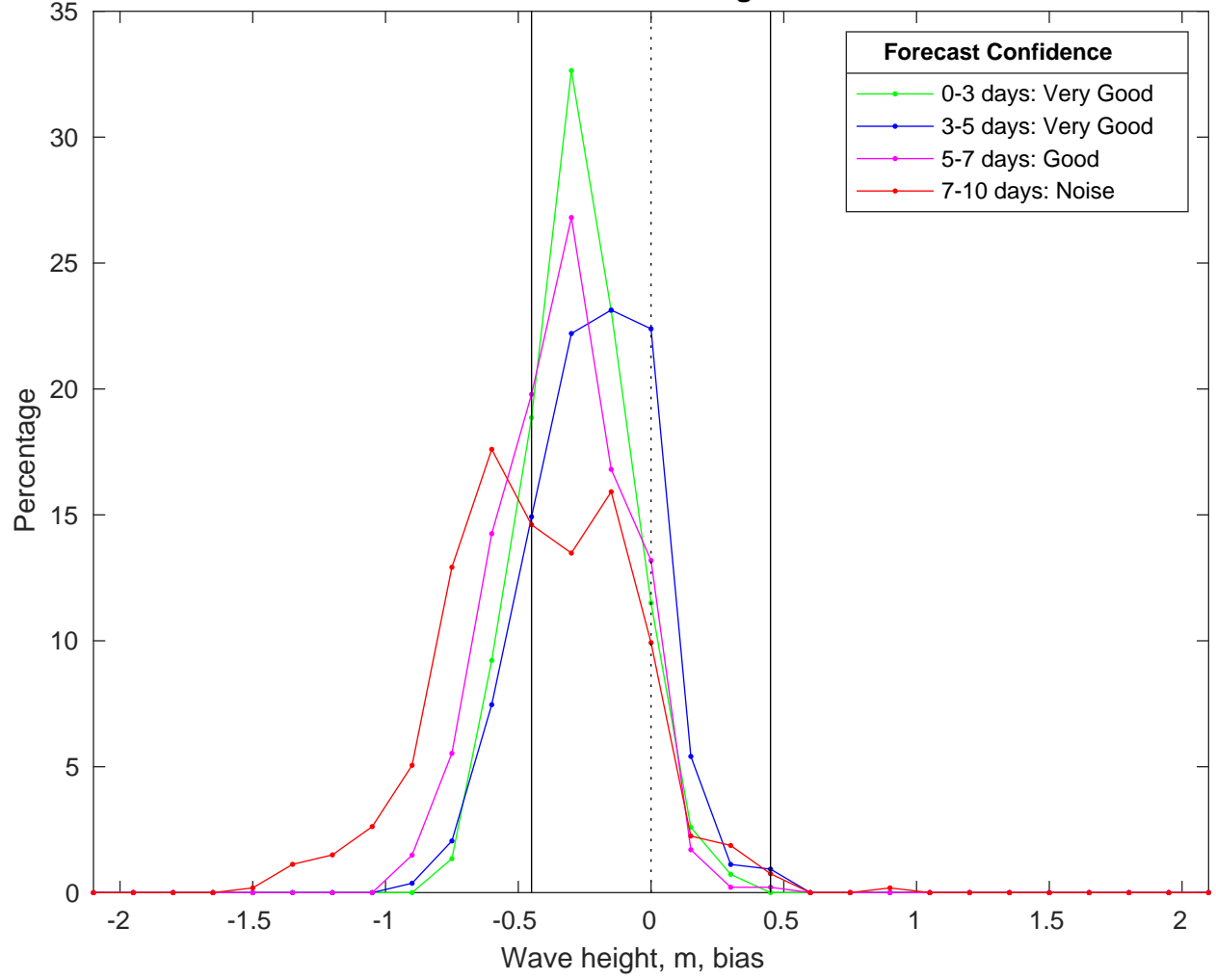
NDBC 52213 vs CMEMS Waves Bias Histogram: 10-Feb-2025
