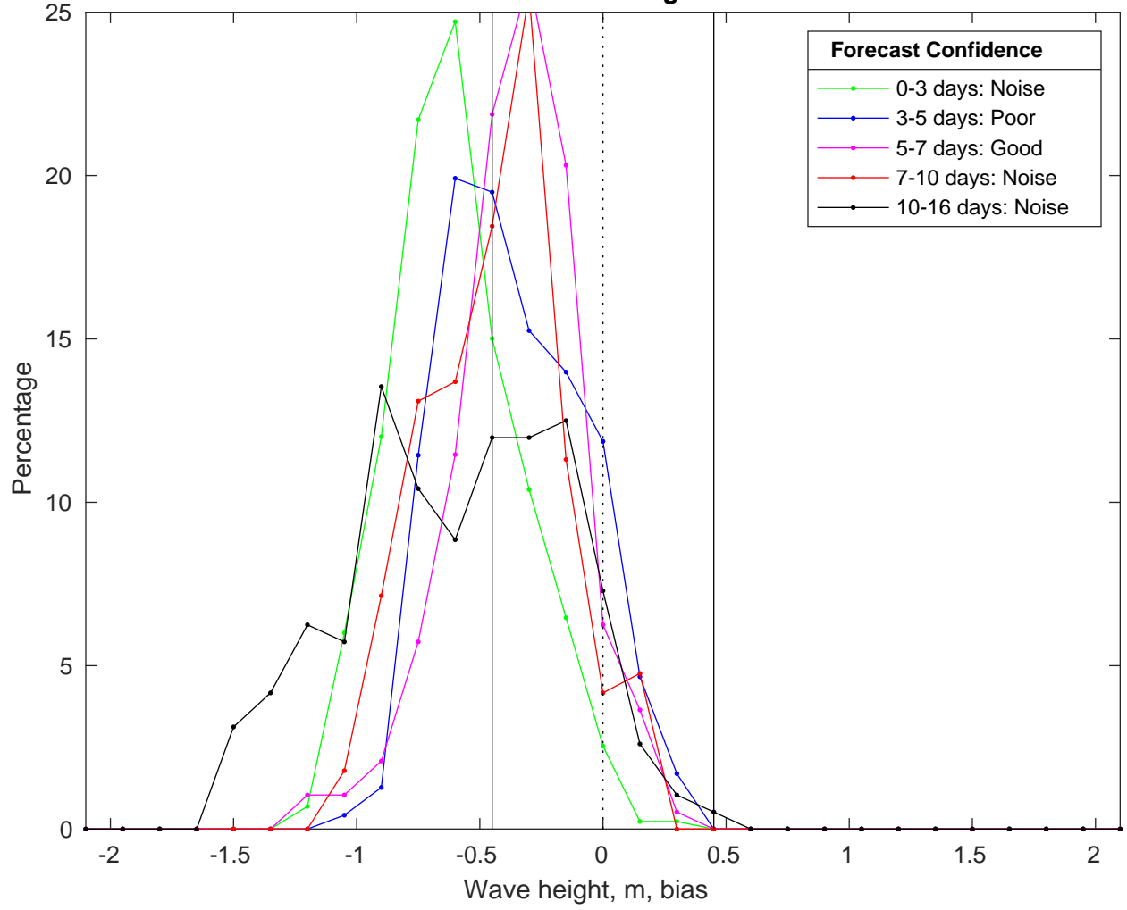
NDBC 52213 vs GFS Waves Bias Histogram: 10-Feb-2025
