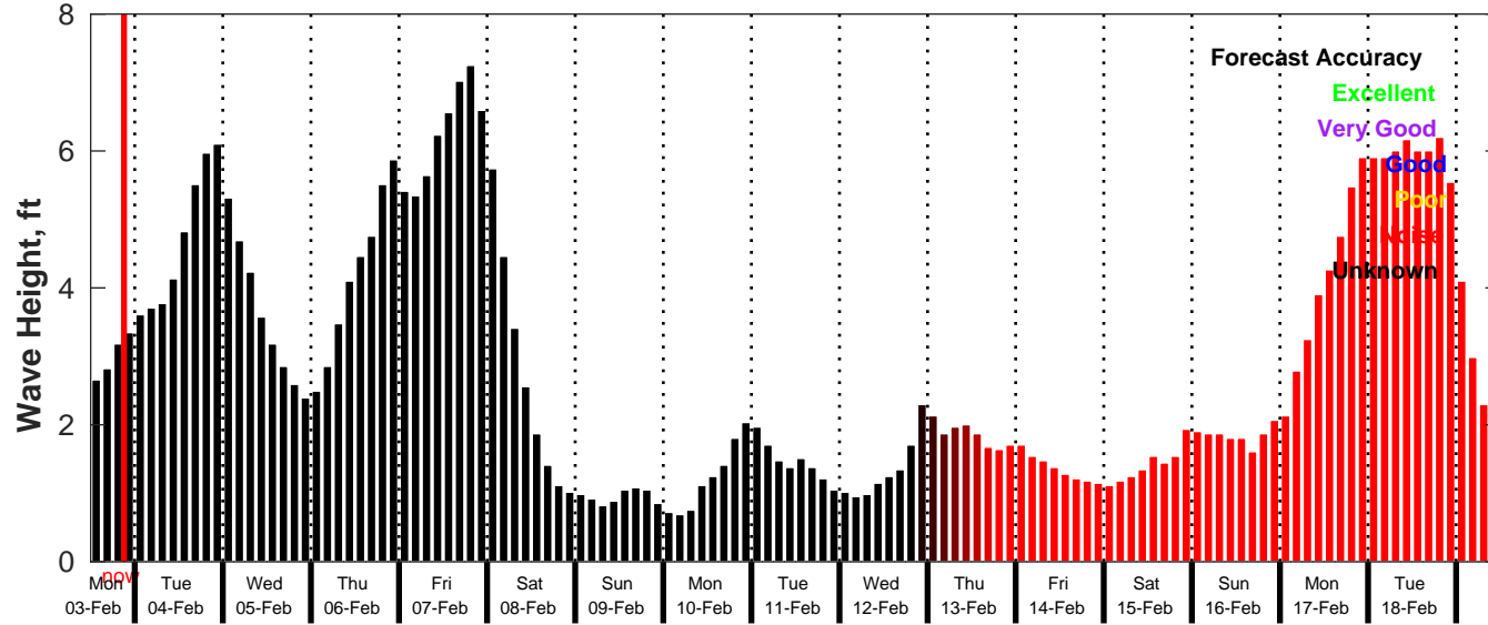
GFS Wave Forecast for NDBC 62305 from 03-Feb-2025 12:00:00 to 19-Feb-2025 12:00:00
