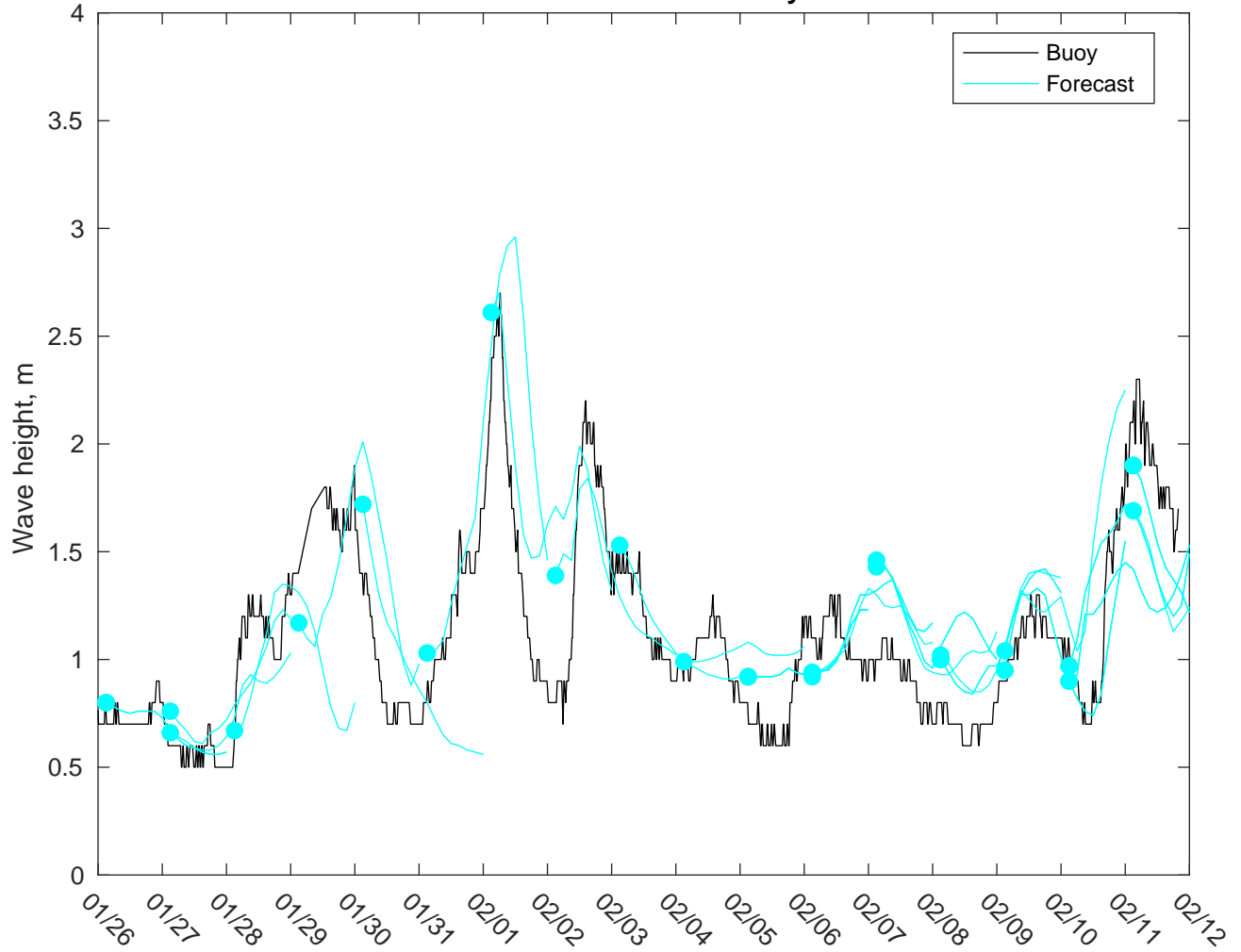
NDBC 41004 vs CMEMS Waves: 5 to 7 day forecast
