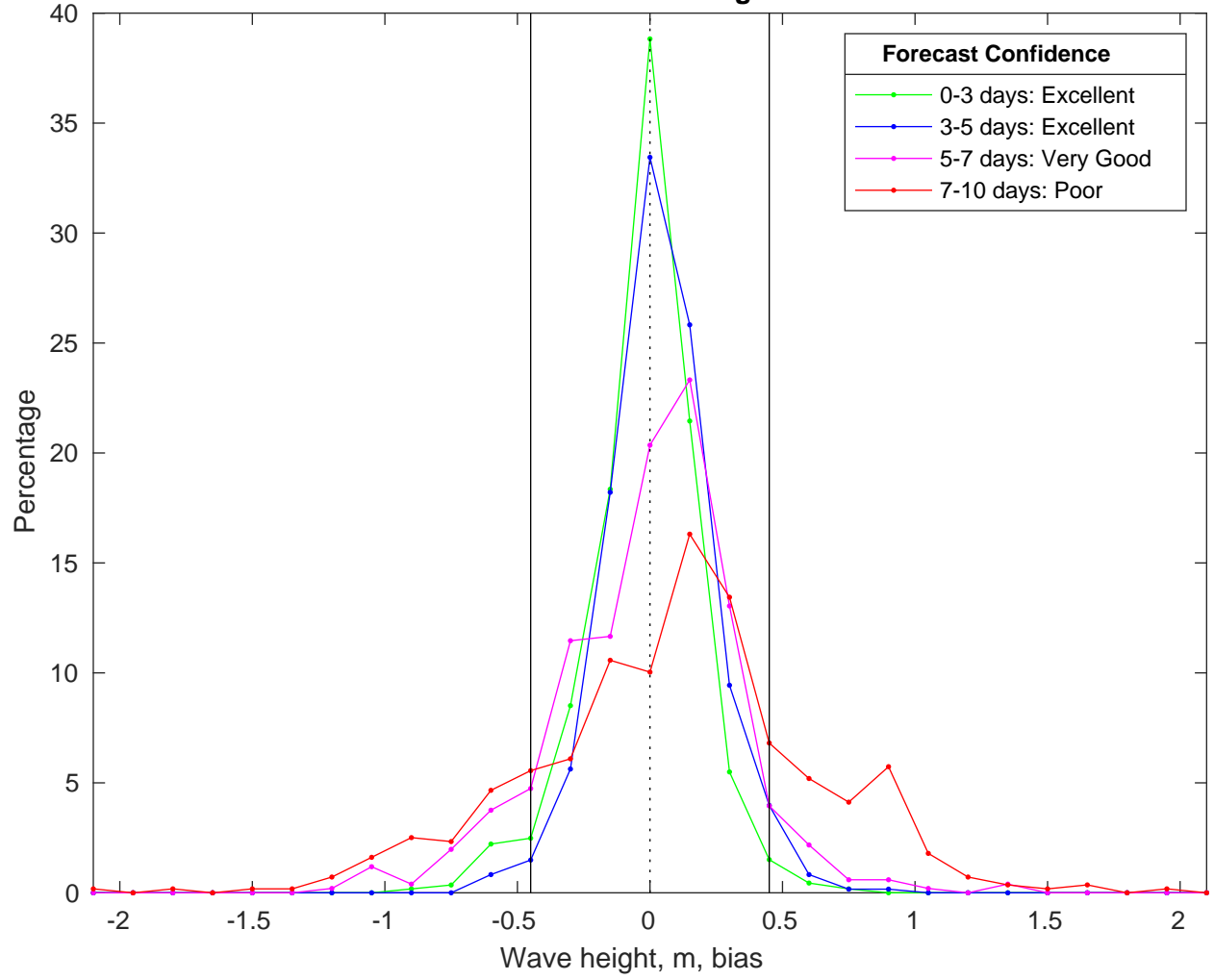
NDBC 41004 vs CMEMS Waves Bias Histogram: 11-Feb-2025
