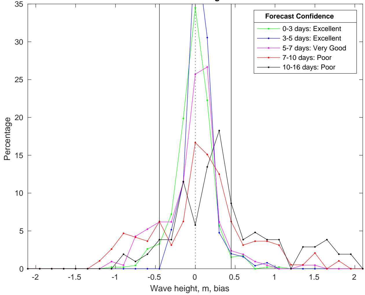
NDBC 41004 vs GFS Waves Bias Histogram: 11-Feb-2025
