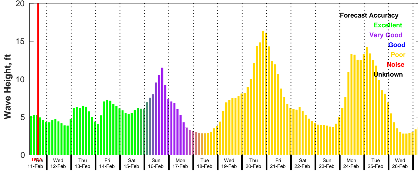
GFS Wave Forecast for NDBC 41004 from 11-Feb-2025 07:00:00 to 27-Feb-2025 07:00:00
