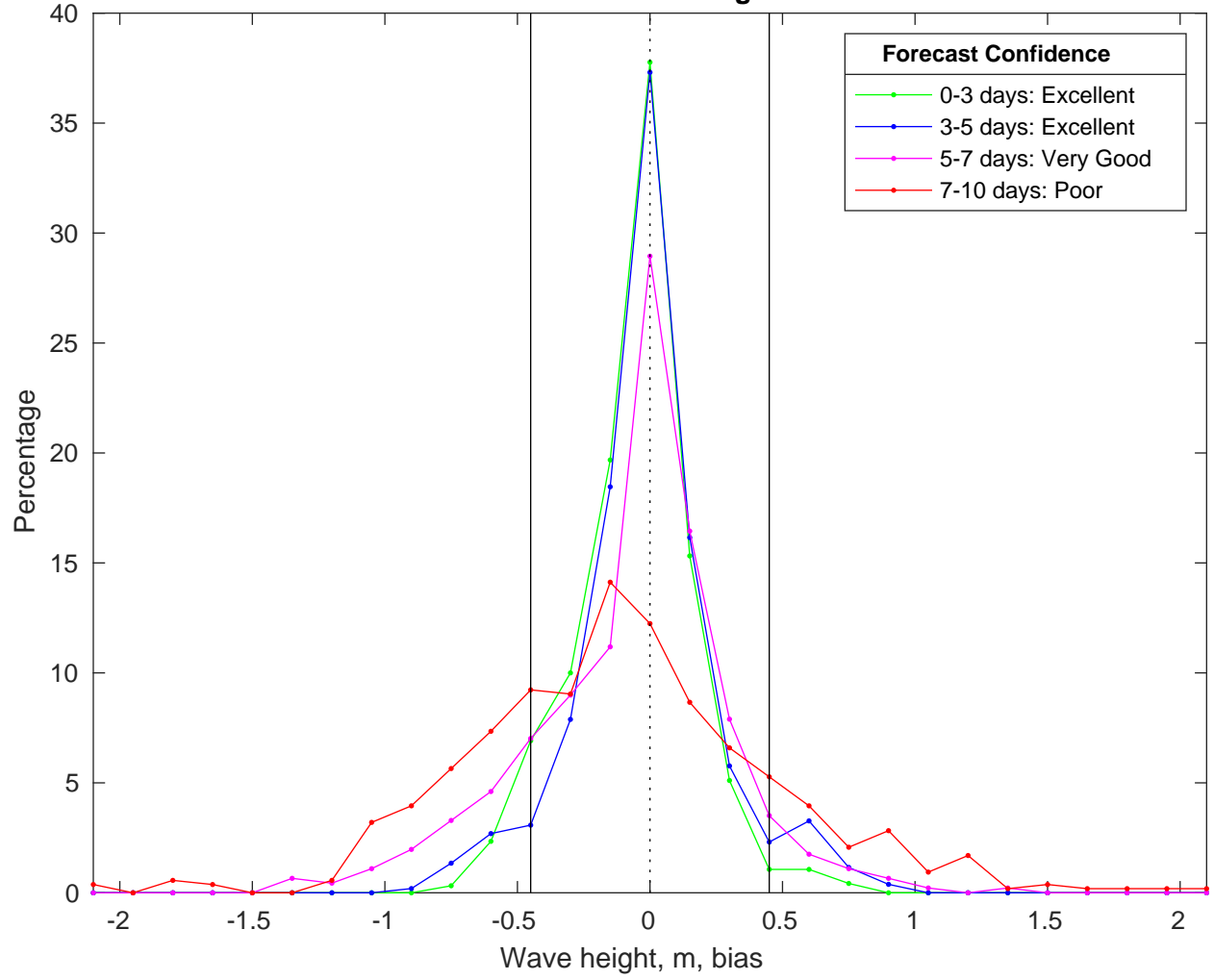
NDBC 41013 vs CMEMS Waves Bias Histogram: 11-Feb-2025
