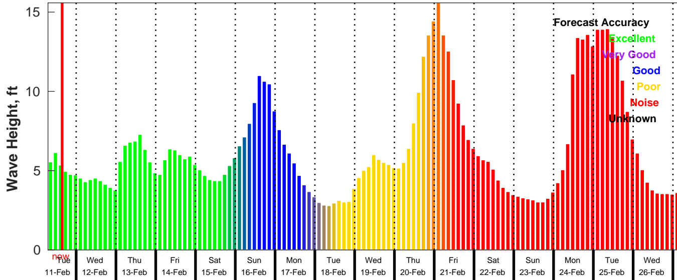
GFS Wave Forecast for NDBC 41013 from 11-Feb-2025 07:00:00 to 27-Feb-2025 07:00:00
