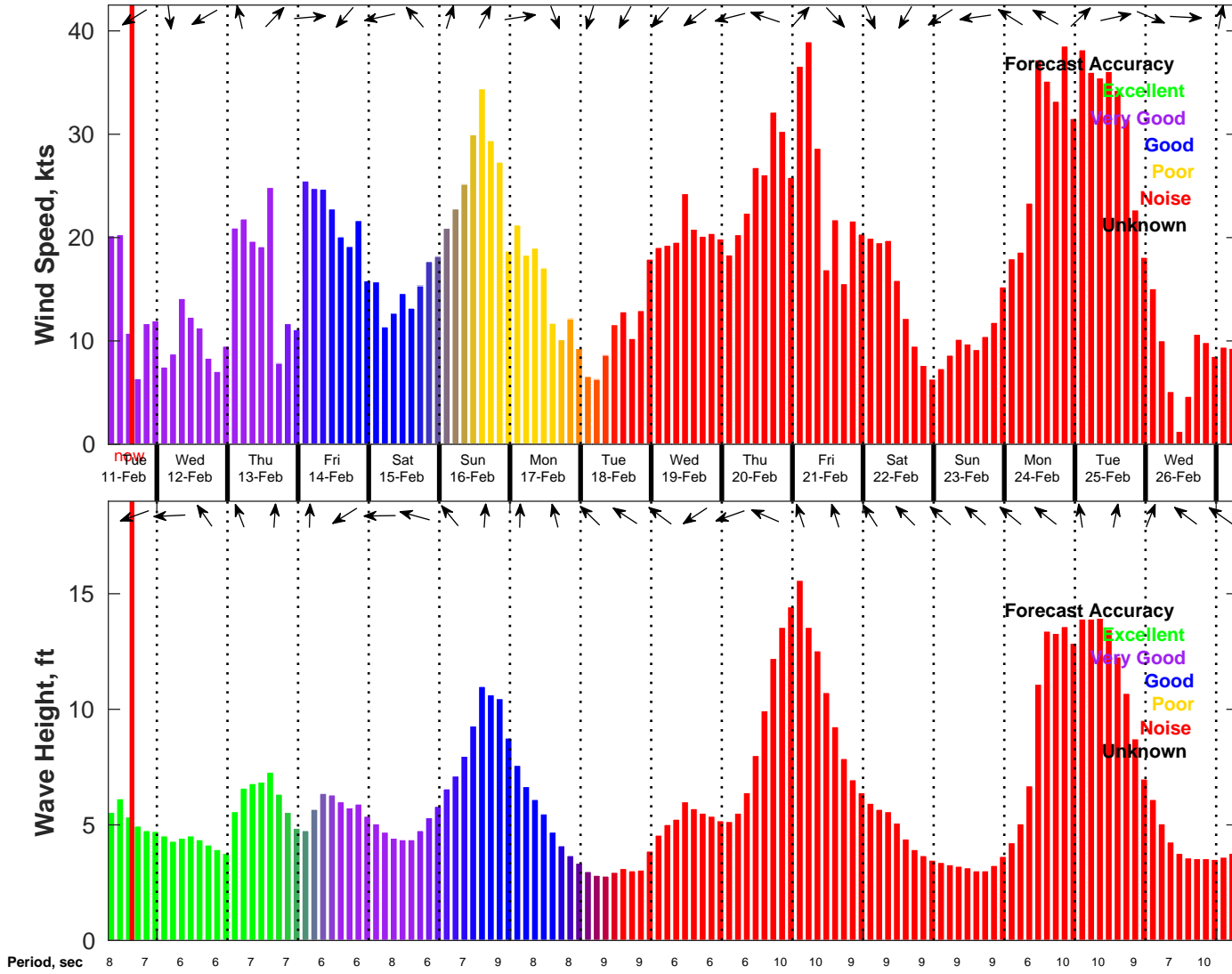
Wind & Wave Forecast for NDBC 41013 from 11-Feb-2025 07:00:00 to 27-Feb-2025 07:00:00
