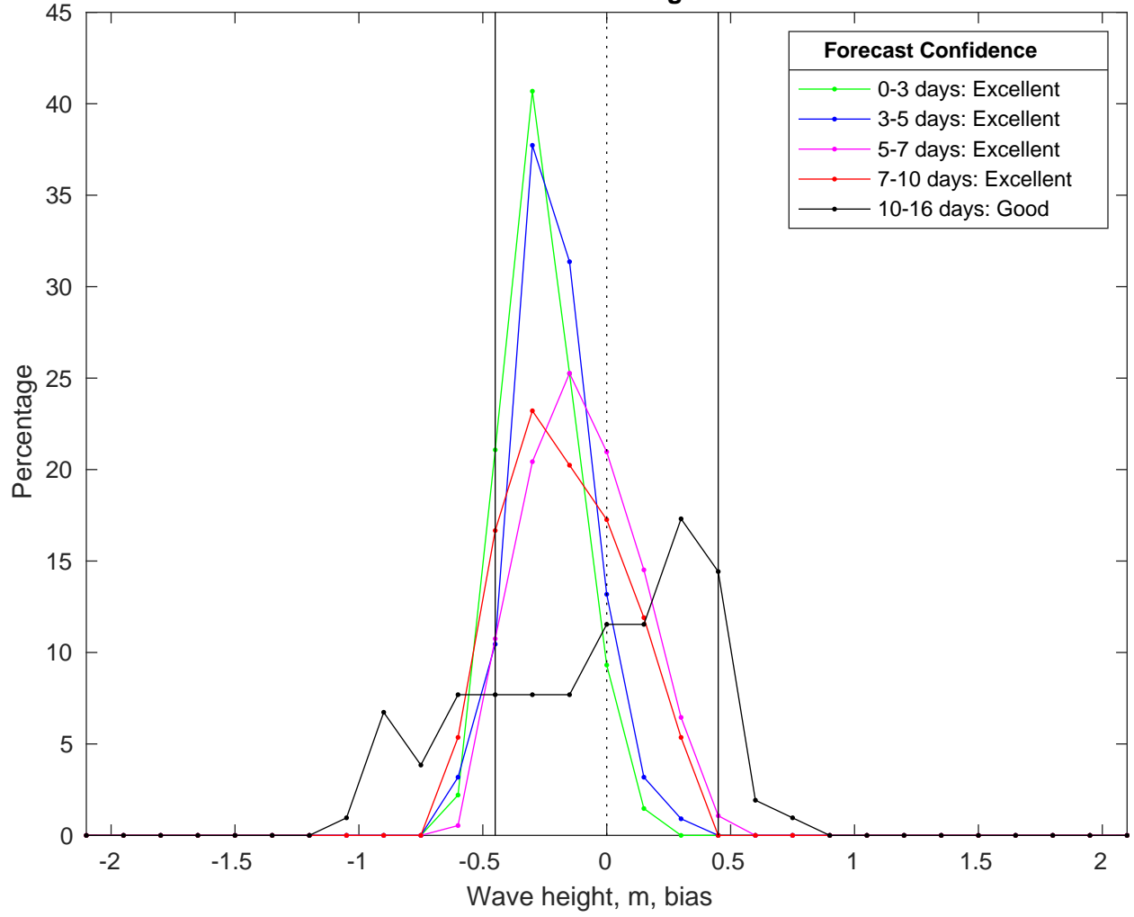
NDBC 41040 vs GFS Waves Bias Histogram: 11-Feb-2025
