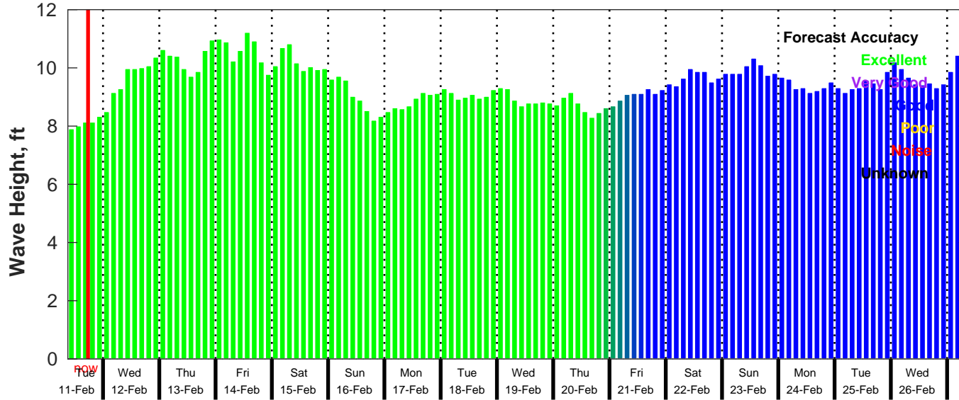
GFS Wave Forecast for NDBC 41040 from 11-Feb-2025 09:00:00 to 27-Feb-2025 09:00:00
