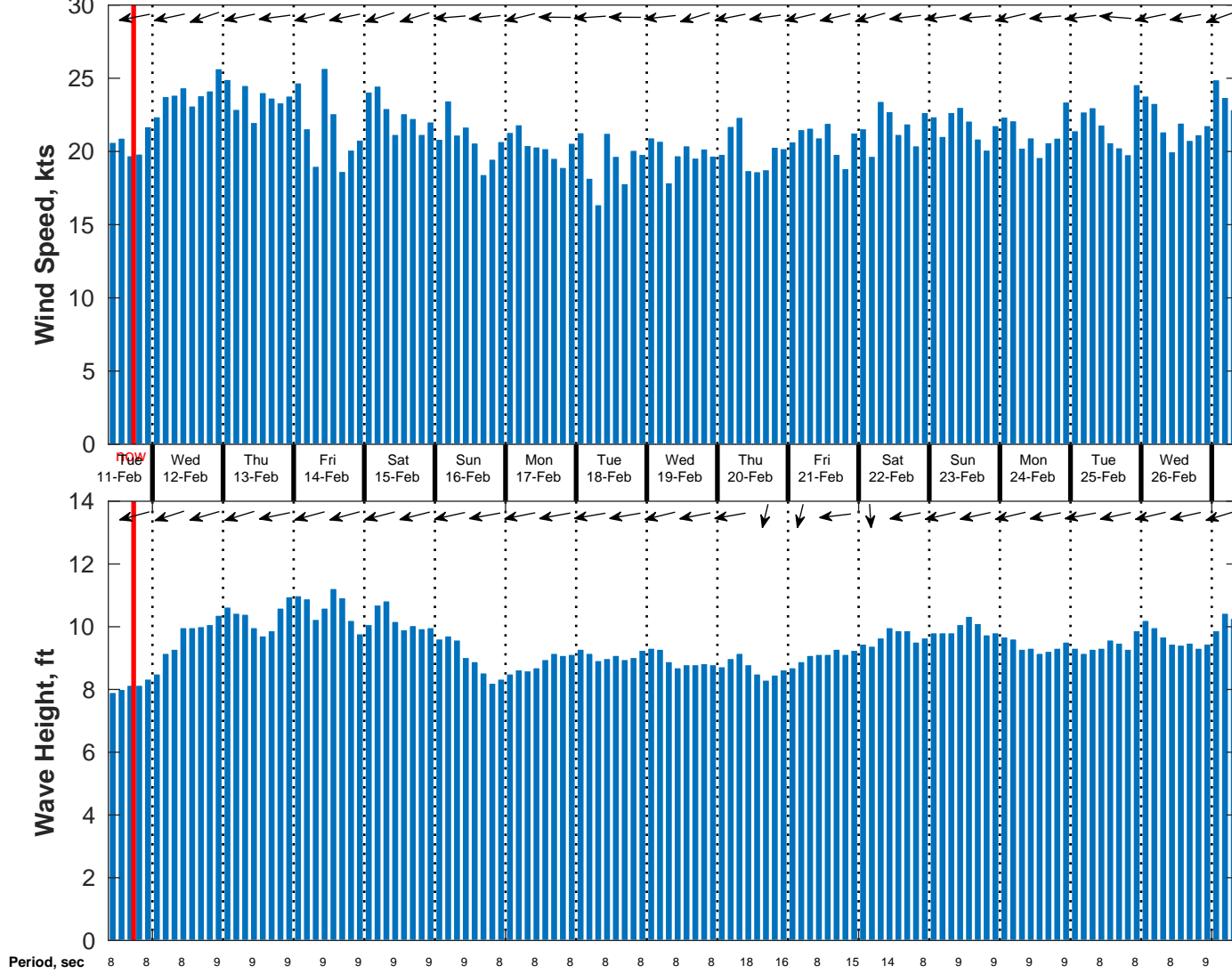
Wind & Wave Forecast for NDBC 41040 from 11-Feb-2025 09:00:00 to 27-Feb-2025 09:00:00
