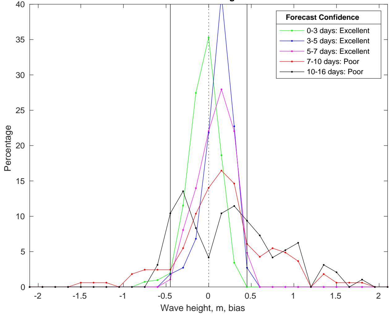
NDBC 42019 vs GFS Waves Bias Histogram: 11-Feb-2025
